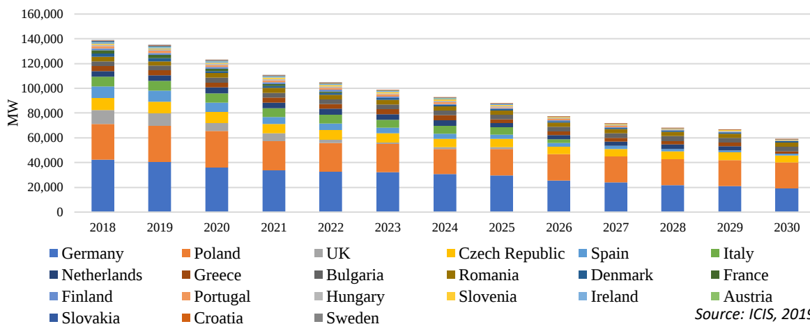
Figure 2: EU coal &amp; lignite capacity by country 2018-2030 (MW)
