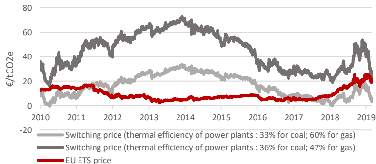
CO2 switching price for different coal and gas power plants efficiencies, in comparison with EU ETS price
